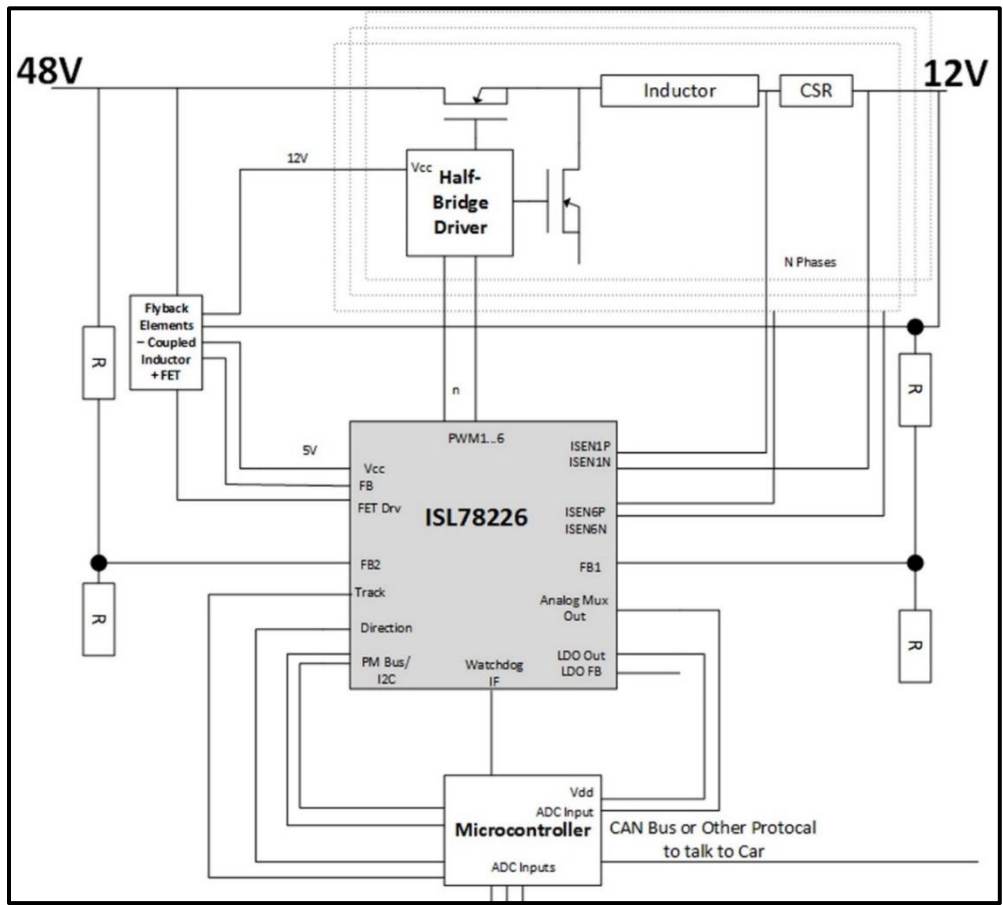
Figure 4. A 3.5kW multiphase 12V/48V system
