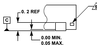
DETAIL "X"
