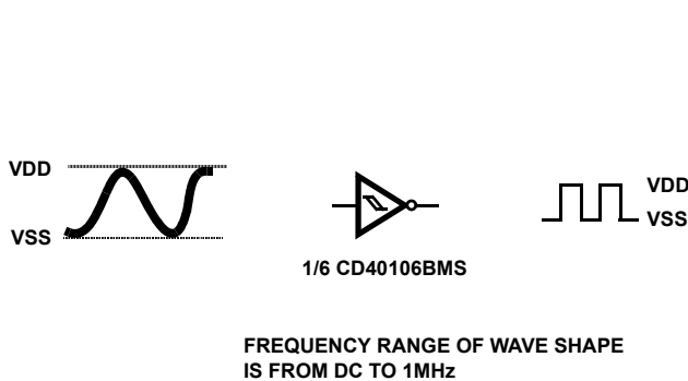
FIGURE 14. WAVE SHAPER
