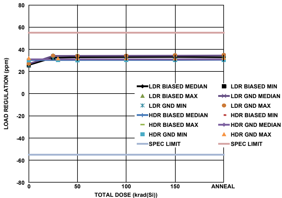
FIGURE 5. ISL71090SEHVF12 load regulation, +20mA sourcing, as a function of total dose irradiation at low and high dose rate for the biased and unbiased cases. The dose rate was 0.01rad(Si)/s for low dose rate irradiation and 68rad(Si)/s for high dose rate irradiation. The irradiations were followed by a biased anneal at 100 °C for 168 hours. Sample sizes were 5 at high dose rate under bias, 5 at high dose rate with all pins grounded, 5 samples at low dose rate under bias and 5 samples at low dose rate with all pins grounded. The SMD post-irradiation specification limit is 55.0ppm/mA maximum.
