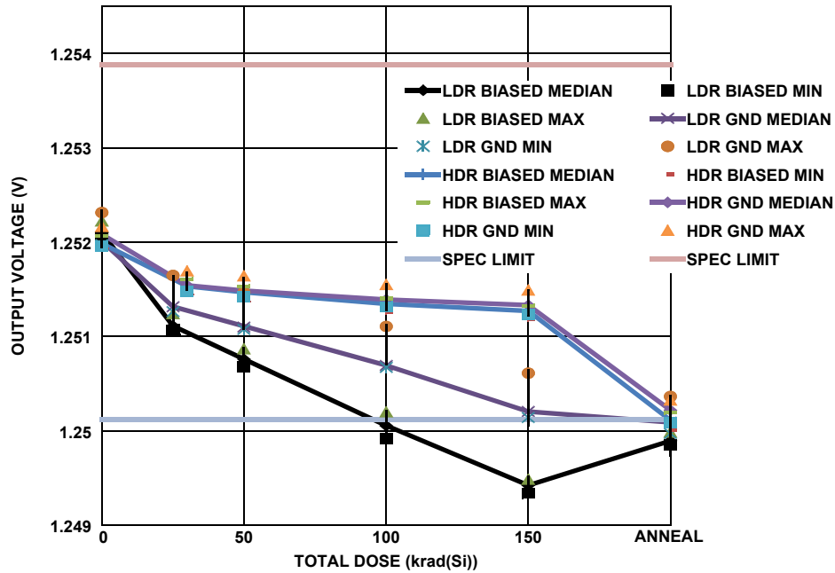
FIGURE 2. ISL71090SEHVF12 output voltage as a function of total dose irradiation at low and high dose rate for the biased (per Figure 1) and unbiased (all pins grounded) cases. The dose rate was 0.01rad(Si)/s for low dose rate irradiation and 68rad(Si)/s for high dose rate irradiation. The irradiations were followed by a biased anneal at 100 °C for 168 hours. Sample sizes were 5 at high dose rate under bias, 5 at high dose rate with all pins grounded, 5 samples at low dose rate under bias and 5 samples at low dose rate with all pins grounded. The SMD post-irradiation specification limits are 1.250122V to 1.253878V.
