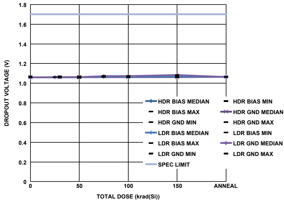
FIGURE 12. ISL71090SEHVF25 dropout voltage as a function of low and high dose rate total dose irradiation for the biased and unbiased cases. The dose rate was 0.01rad(Si)/s for low dose rate irradiation and 68rad(Si)/s for high dose rate irradiation. The irradiations were followed by a biased anneal at 100 °C for 168 hours. Sample sizes were 7 at high dose rate under bias, 7 at high dose rate with all pins grounded, 5 samples at low dose rate under bias and 5 samples at low dose rate with all pins grounded. The post-irradiation specification limit is 1.7V maximum.
