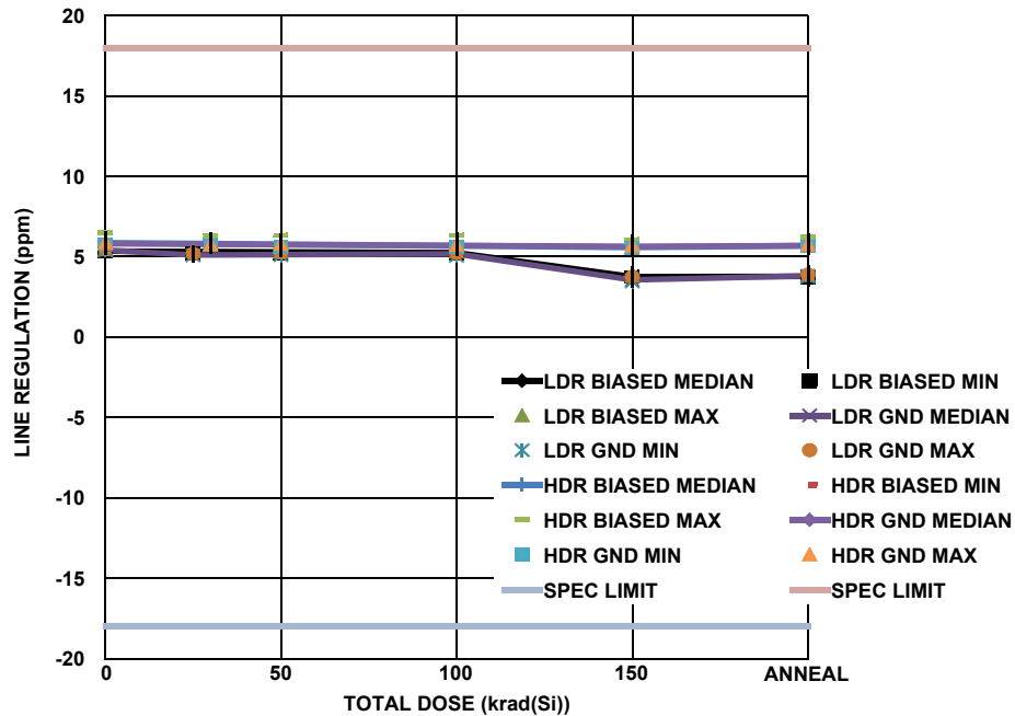
FIGURE 4. ISL71090SEHVF12 line regulation as a function of total dose irradiation at low and high dose rate for the biased and unbiased cases. The dose rate was 0.01rad(Si)/s for low dose rate irradiation and 68rad(Si)/s for high dose rate irradiation. The irradiations were followed by a biased anneal at 100 °C for 168 hours. Sample sizes were 5 at high dose rate under bias, 5 at high dose rate with all pins grounded, 5 samples at low dose rate under bias and 5 samples at low dose rate with all pins grounded. The SMD post-irradiation specification limit is 18.0ppm/V maximum.
