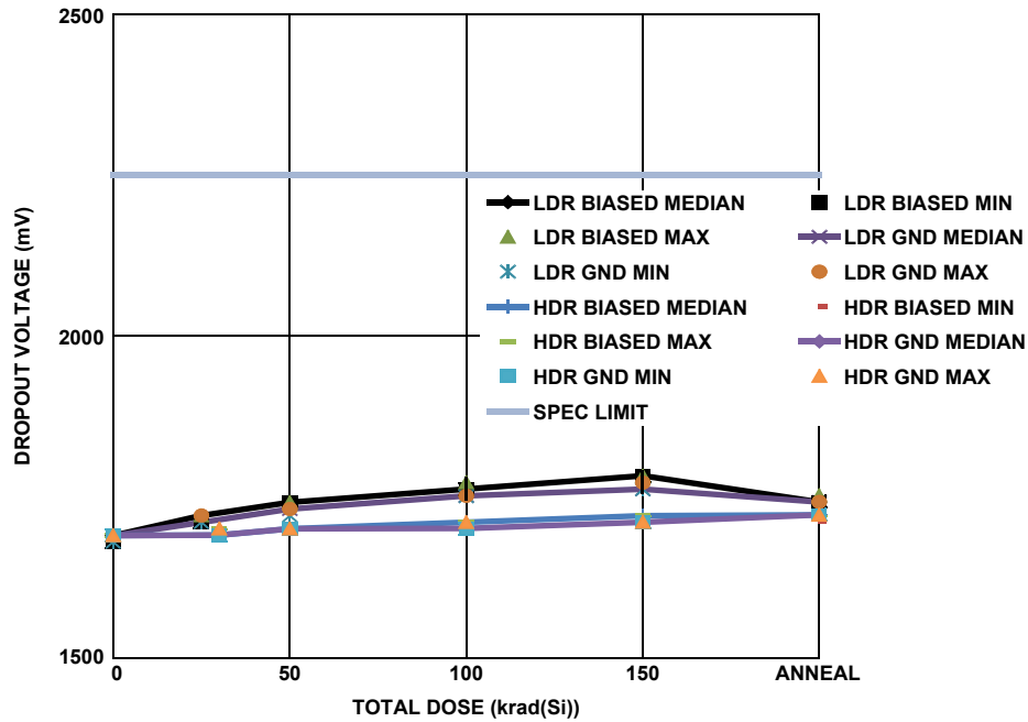
FIGURE 6. ISL71090SEHVF12 dropout voltage as a function of total dose irradiation at low and high dose rate for the biased and unbiased cases. The dose rate was 0.01rad(Si)/s for low dose rate irradiation and 68rad(Si)/s for high dose rate irradiation. The irradiations were followed by a biased anneal at 100 °C for 168 hours. Sample sizes were 5 at high dose rate under bias, 5 at high dose rate with all pins grounded, 5 samples at low dose rate under bias and 5 samples at low dose rate with all pins grounded. The post-irradiation specification limit is 2250mV maximum.
