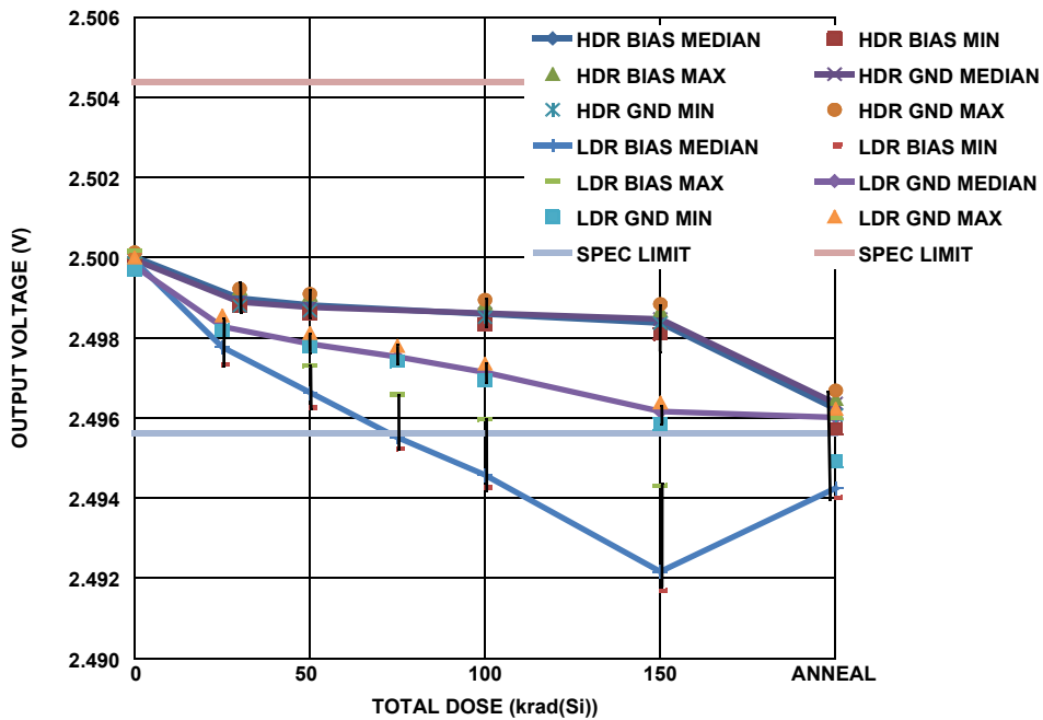
FIGURE 7. ISL71090SEHVF25 output voltage as a function of total dose irradiation at low and high dose rate for the biased and unbiased cases. The dose rate was 0.01rad(Si)/s for low dose rate irradiation and 68rad(Si)/s for high dose rate irradiation. The irradiations were followed by a biased anneal at 100 °C for 168 hours. Sample sizes were 7 at high dose rate under bias, 7 at high dose rate with all pins grounded, 5 samples at low dose rate under bias and 5 samples at low dose rate with all pins grounded. The SMD post-irradiation specification limits are 2.495625V to 2.504375V.
