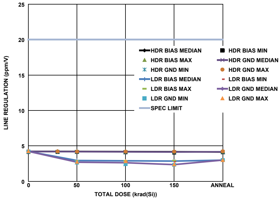
FIGURE 15. ISL71090SEHVF50 line regulation as a function of high dose rate total dose irradiation for the biased and unbiased cases. The dose rate was 0.01rad(Si)/s for low dose rate irradiation and 68rad(Si)/s for high dose rate irradiation. The irradiations were followed by a biased anneal at 100 °C for 168 hours. Sample sizes were 5 at high dose rate under bias, 5 at high dose rate with all pins grounded, 2 samples at low dose rate under bias and 2 samples at low dose rate with all pins grounded. The SMD post-irradiation specification limit is 20ppm/V maximum.
