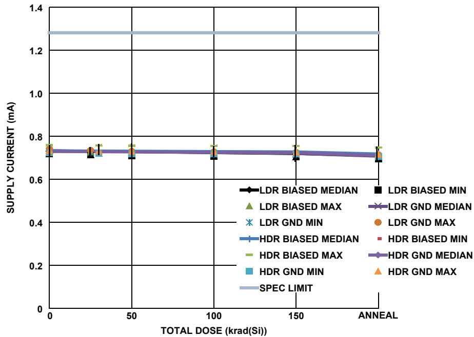
FIGURE 3. ISL71090SEHVF12 power supply current as a function of total dose irradiation at low and high dose rate for the biased and unbiased cases. The dose rate was 0.01rad(Si)/s for low dose rate irradiation and 68rad(Si)/s for high dose rate irradiation. The irradiations were followed by a biased anneal at 100 °C for 168 hours. Sample sizes were 5 at high dose rate under bias, 5 at high dose rate with all pins grounded, 5 samples at low dose rate under bias and 5 samples at low dose rate with all pins grounded. The SMD post-irradiation specification limit is 1.28mA maximum.
