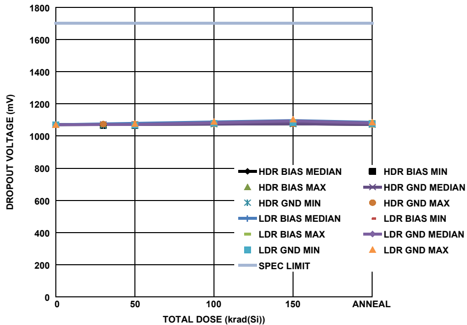
FIGURE 18. ISL71090SEHVF50 dropout voltage as a function of high dose rate total dose irradiation for the biased and unbiased cases. The dose rate was 0.01rad(Si)/s for low dose rate irradiation and 68rad(Si)/s for high dose rate irradiation. The irradiations were followed by a biased anneal at 100 °C for 168 hours. Sample sizes were 5 at high dose rate under bias, 5 at high dose rate with all pins grounded, 2 samples at low dose rate under bias and 2 samples at low dose rate with all pins grounded. The SMD post-irradiation specification limit is 1700mV maximum.
