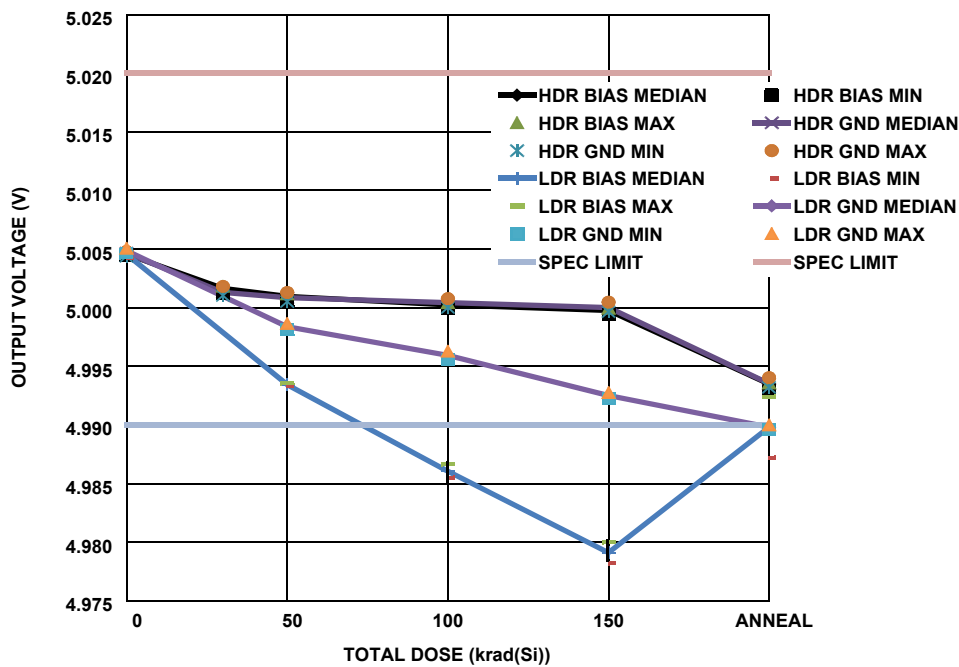
FIGURE 13. ISL71090SEHVF50 output voltage as a function of high dose rate total dose irradiation for the biased and unbiased cases. The dose rate was 0.01rad(Si)/s for low dose rate irradiation and 68rad(Si)/s for high dose rate irradiation. The irradiations were followed by a biased anneal at 100 °C for 168 hours. Sample sizes were 5 at high dose rate under bias, 5 at high dose rate with all pins grounded, 2 samples at low dose rate under bias and 2 samples at low dose rate with all pins grounded. The SMD post-irradiation specification limits are 4.989985V to 5.020015V.
