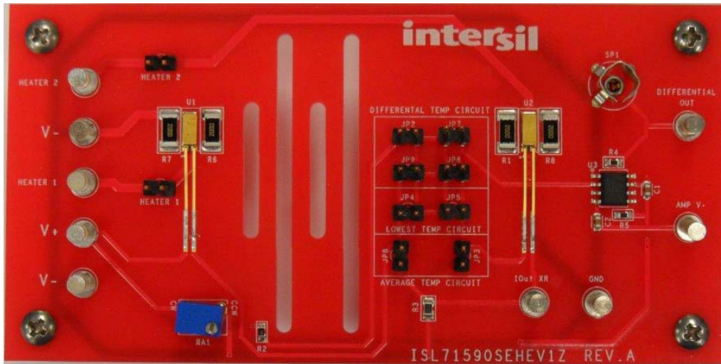
FIGURE 1. ISL71590SEHEV1Z EVALUATION BOARD
