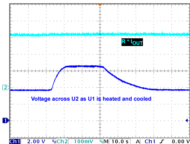
FIGURE 5. ISL71590SEH IN SERIES CONFIGURATION SHOWING VOLTAGE AROSS COOLER SENSOR
