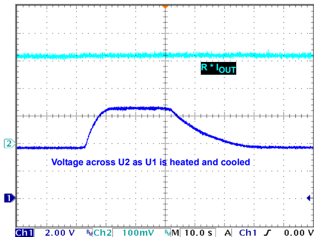
FIGURE 5. ISL71590SEH IN SERIES CONFIGURATION SHOWING VOLTAGE ACROSS COOLER SENSOR
