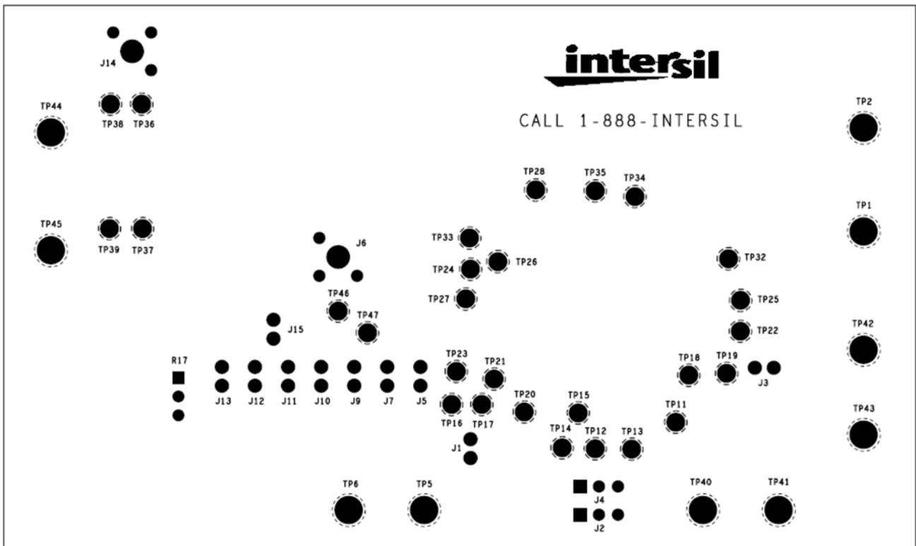
FIGURE 7. SILK SCREEN BOTTOM
