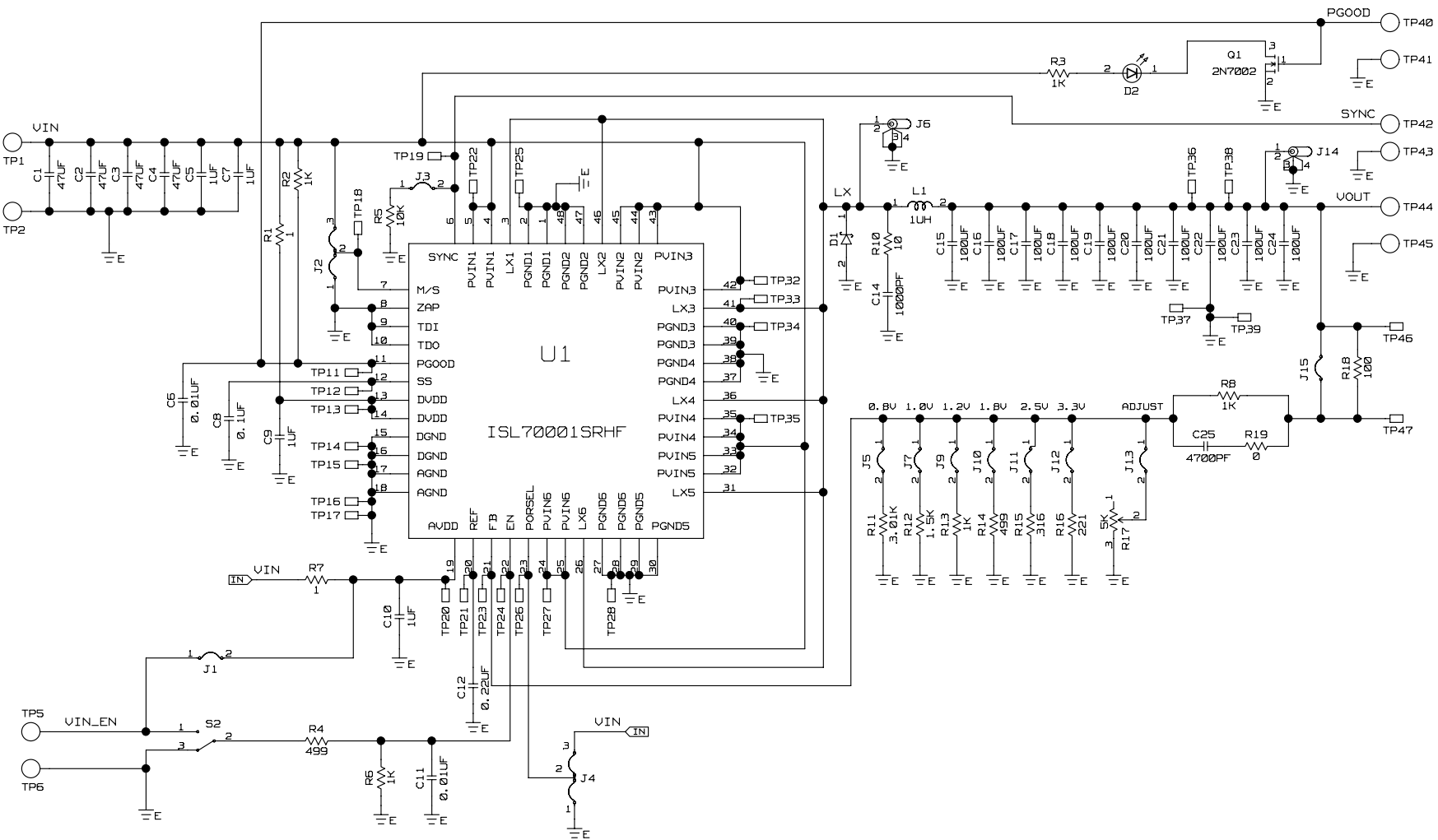
FIGURE 1. ISL70001SRHEVAL1Z SCHEMATIC
