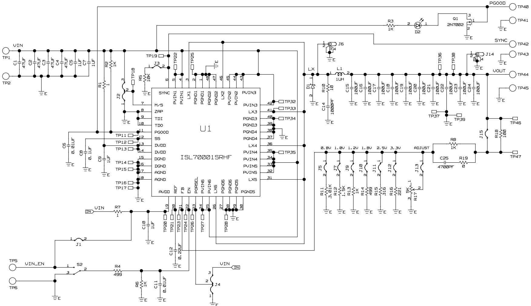
FIGURE 1. ISL70001SRHEVAL1Z SCHEMATIC
