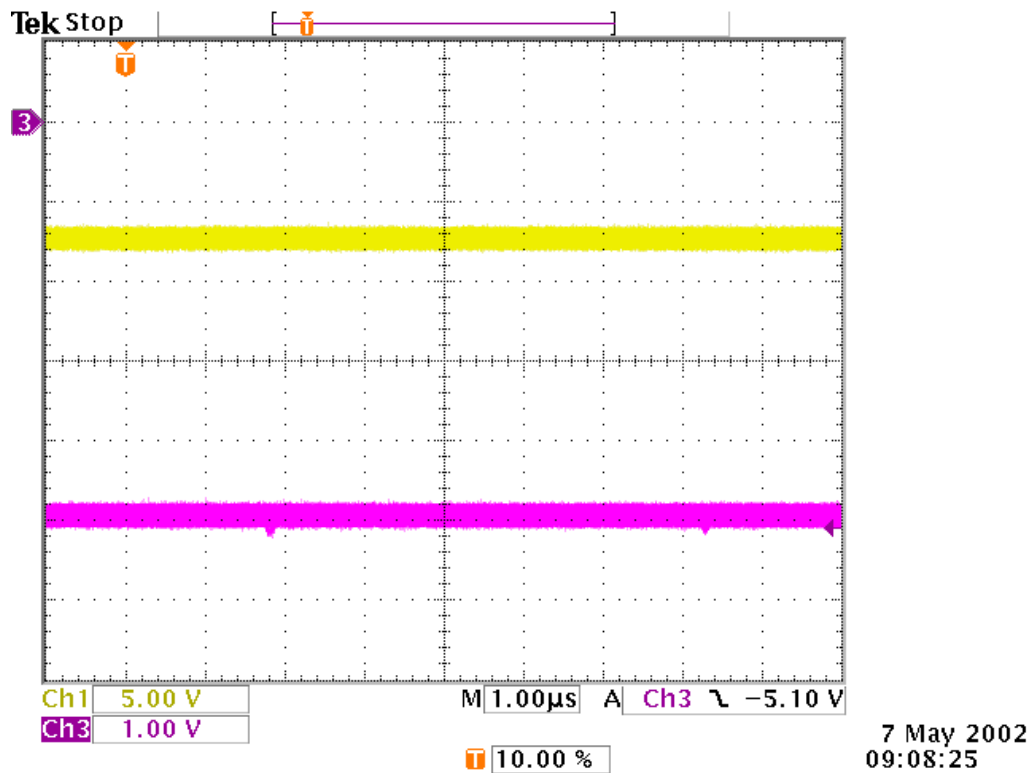
Figure 32: Test #32 Results ( V_{in} = -7V ; V_{out} = -5V ; I_{out} = 3.75mA ; C_{out} = 44\mu F )
