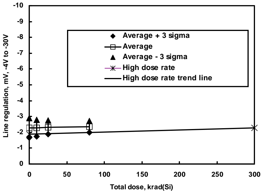
Figure 6: ISL72991RH line regulation as a function of total dose, low and high dose rate (.01rad(Si)/s and 120rad(Si)/s). Plot shows output voltage change for an input voltage change from -4V to -30V. Sample size is 13 parts. The minimum post-radiation output voltage change specification is +/-25mV.
