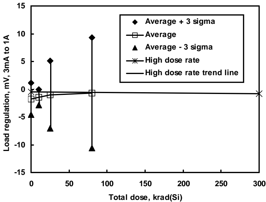
Figure 7: ISL72991RH load regulation as a function of total dose, low and high dose rate (.01rad(Si)/s and 120rad(Si)/s). The plot shows output voltage change for an output current change from 3mA to 1A. Sample size is 13 parts. The minimum post-radiation output voltage change specification is +/-12mV.
