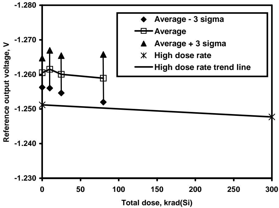
Figure 3: ISL72991RH reference output voltage as a function of total dose, low and high dose rate (.01rad(Si)/s and 120rad(Si)/s). Sample size is 13 parts. The maximum voltage range specification is -1.279 to -1.231 V.
