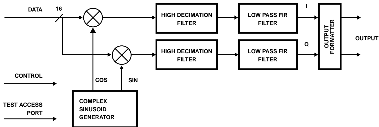
FIGURE 6. BLOCK DIAGRAM OF HSP50016 DIGITAL DOWN CONVERTER
