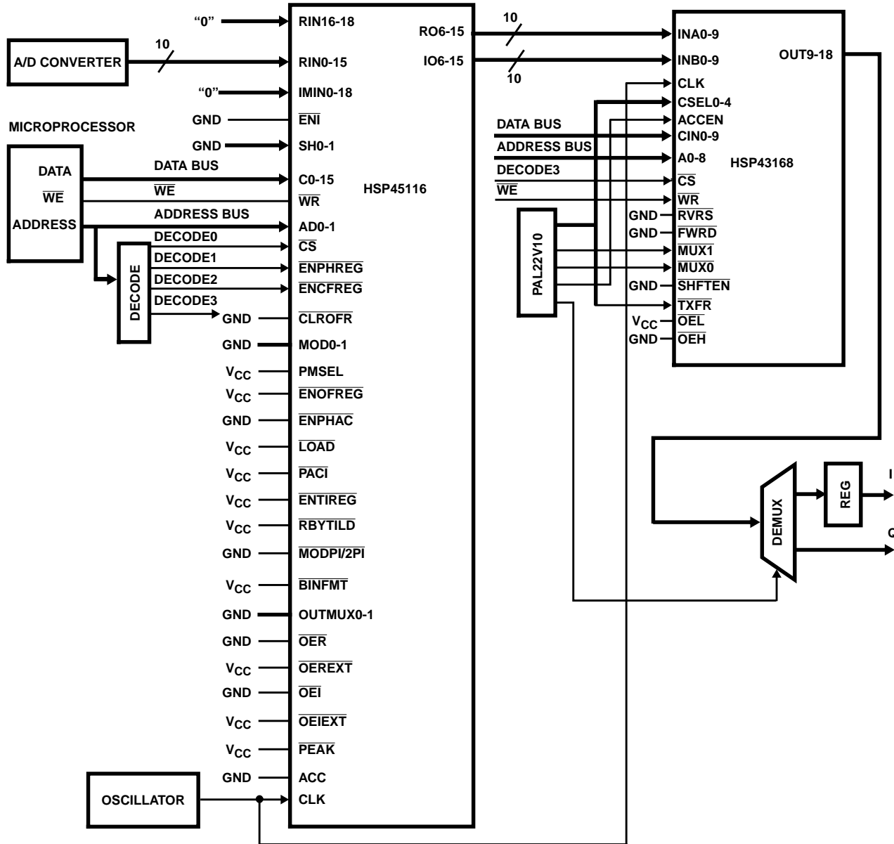
FIGURE 4. FUNCTIONAL BLOCK DIAGRAM FOR WIDE BAND DOWN CONVERSION WITH HSP45116 AND HSP43168
