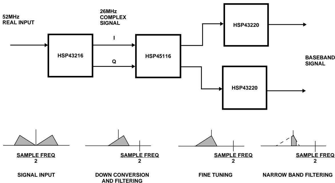
FIGURE 7. HALF BAND FILTER IN QUADRATURE DOWN CONVERSION
