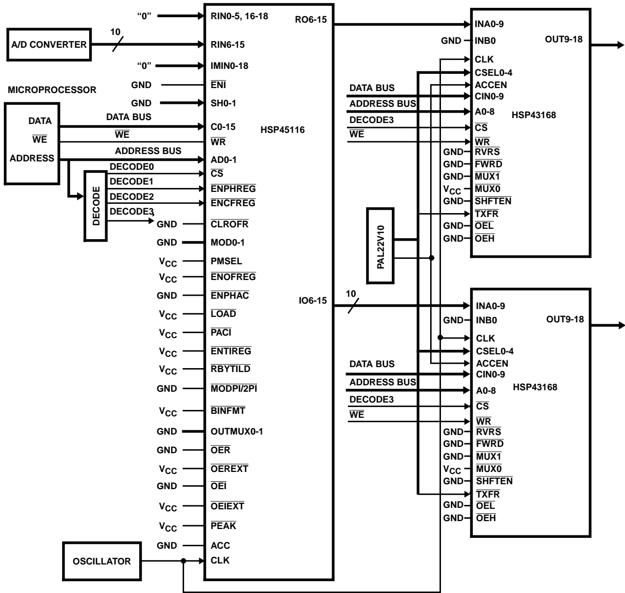
FIGURE 3. FUNCTIONAL BLOCK DIAGRAM FOR WIDE BAND QUADRATURE DOWN CONVERSION WITH HSP45116 AND HSP43168
