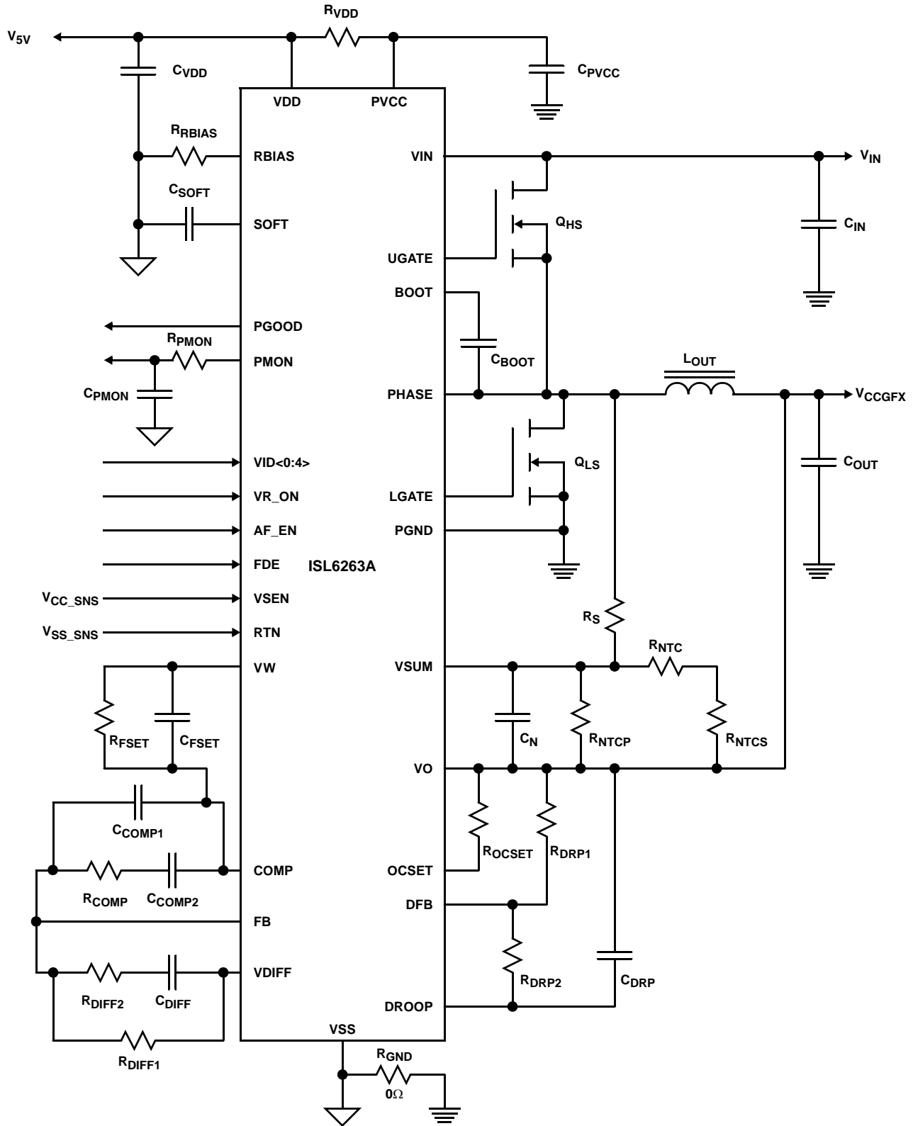
FIGURE 2. ISL6263A GPU RENDER-CORE VOLTAGE REGULATOR SOLUTION WITH DCR CURRENT SENSING
