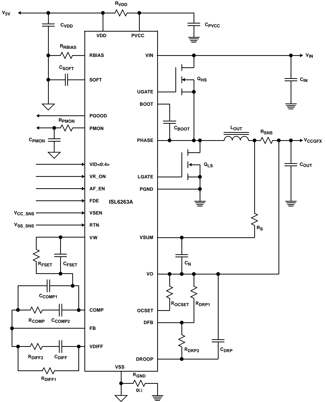
FIGURE 3. ISL6263A GPU RENDER-CORE VOLTAGE REGULATOR SOLUTION WITH RESISTIVE CURRENT SENSING
