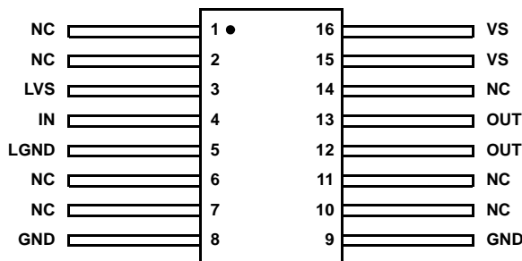
ISL74422ARH-F (FLATPACK CDFF4-F16) TOP VIEW
