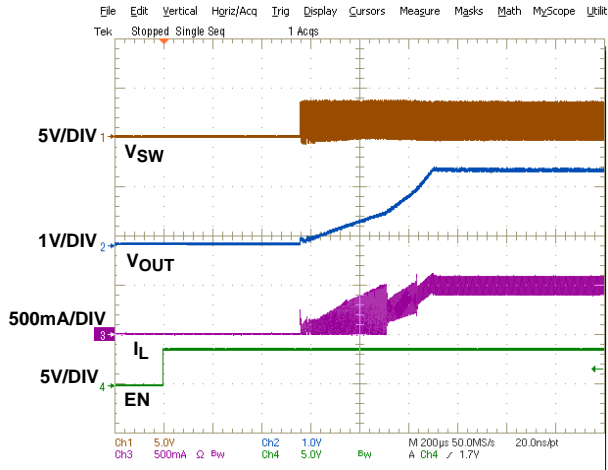
FIGURE 7. SOFT-START TO PWM MODE ( V_{IN} = 3.6V , V_{OUT} = 1.5V , I_{OUT} = 500mA )
