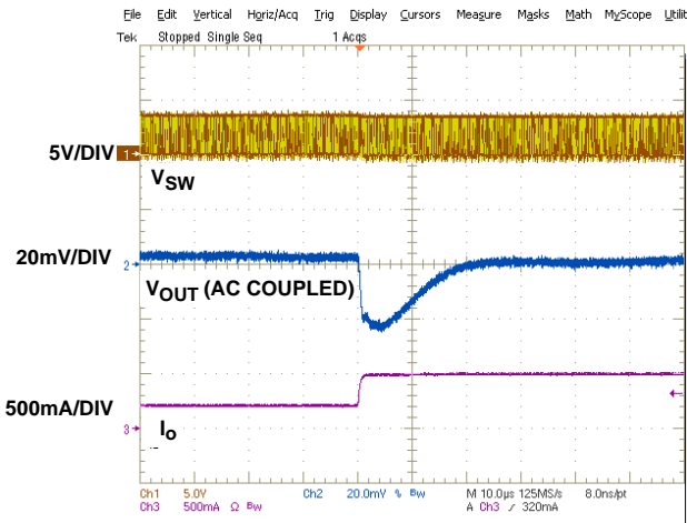
FIGURE 19. LOAD TRANSIENT IN PWM MODE ( V_{IN} = 3.6V , V_O = 2.5V , 200mA TO 500mA)
