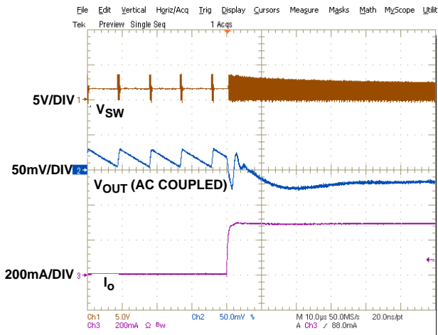
FIGURE 13. LOAD TRANSIENT FROM PFM TO PWM MODE ( V_{IN} = 3.6V , V_{OUT} = 1.5V , 5mA TO 300mA)
