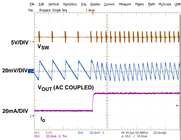
FIGURE 9. LOAD TRANSIENT IN PFM MODE ( V_{IN} = 3.6V , V_{OUT} = 1.5V , 5mA TO 30mA)
