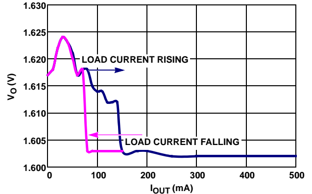
FIGURE 4. OUTPUT VOLTAGE vs LOAD CURRENT ( V_{IN} = 3.6\text{V} , V_{OUT} = 1.6\text{V} )
