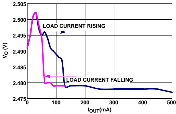
FIGURE 5. OUTPUT VOLTAGE vs LOAD CURRENT ( V_{IN} = 4.0V , V_{OUT} = 2.5V )
