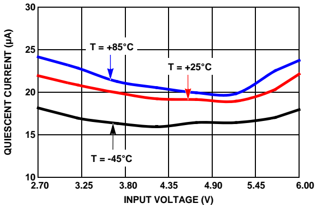
FIGURE 3. INPUT QUIESCENT CURRENT vs V_{IN} ( V_{OUT} = 2.5\text{V} )
