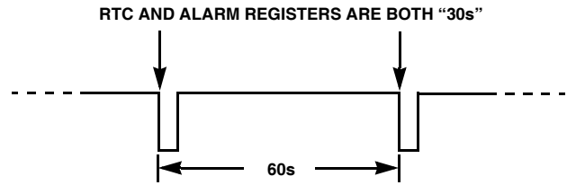
FIGURE 14. \overline{IRQ}/F_{OUT} WAVEFORM
