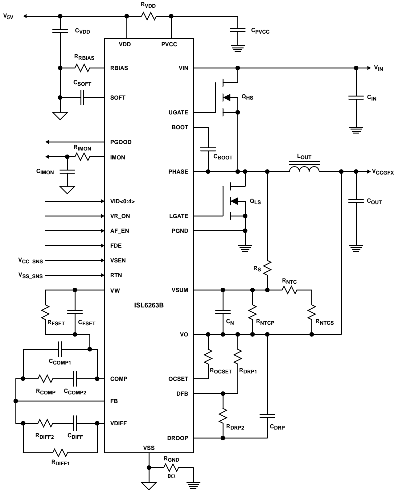
FIGURE 2. ISL6263B GPU RENDER-CORE VOLTAGE REGULATOR SOLUTION WITH DCR CURRENT SENSING
