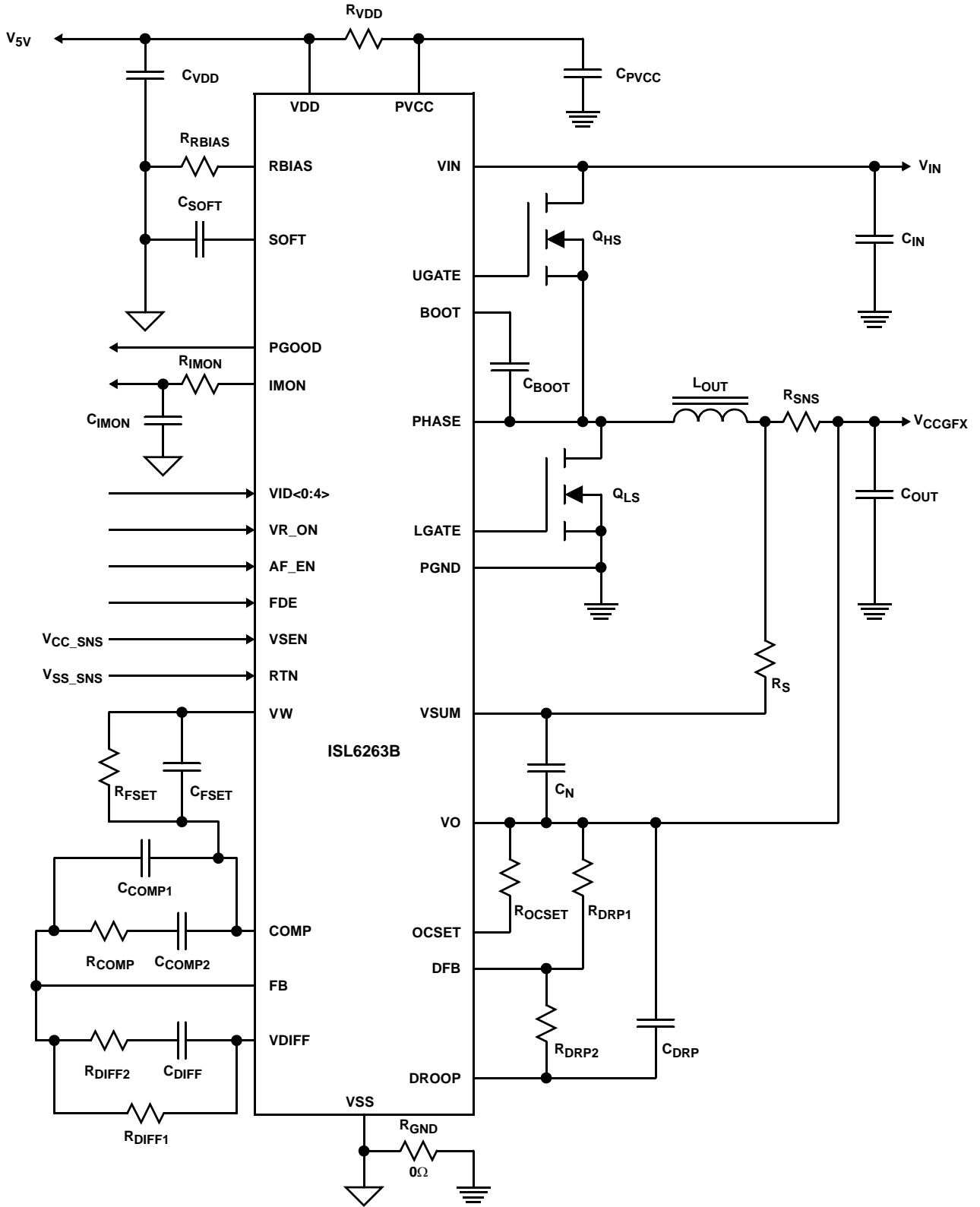
FIGURE 3. ISL6263B GPU RENDER-CORE VOLTAGE REGULATOR SOLUTION WITH RESISTIVE CURRENT SENSING
