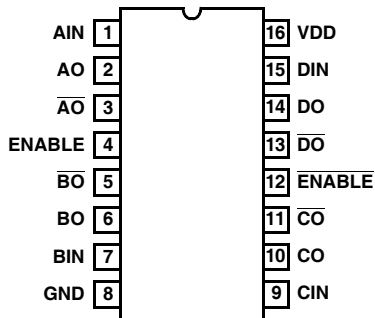
HS9-26C31RH (16 LD FLATPACK) CDFP4-F16 TOP VIEW
