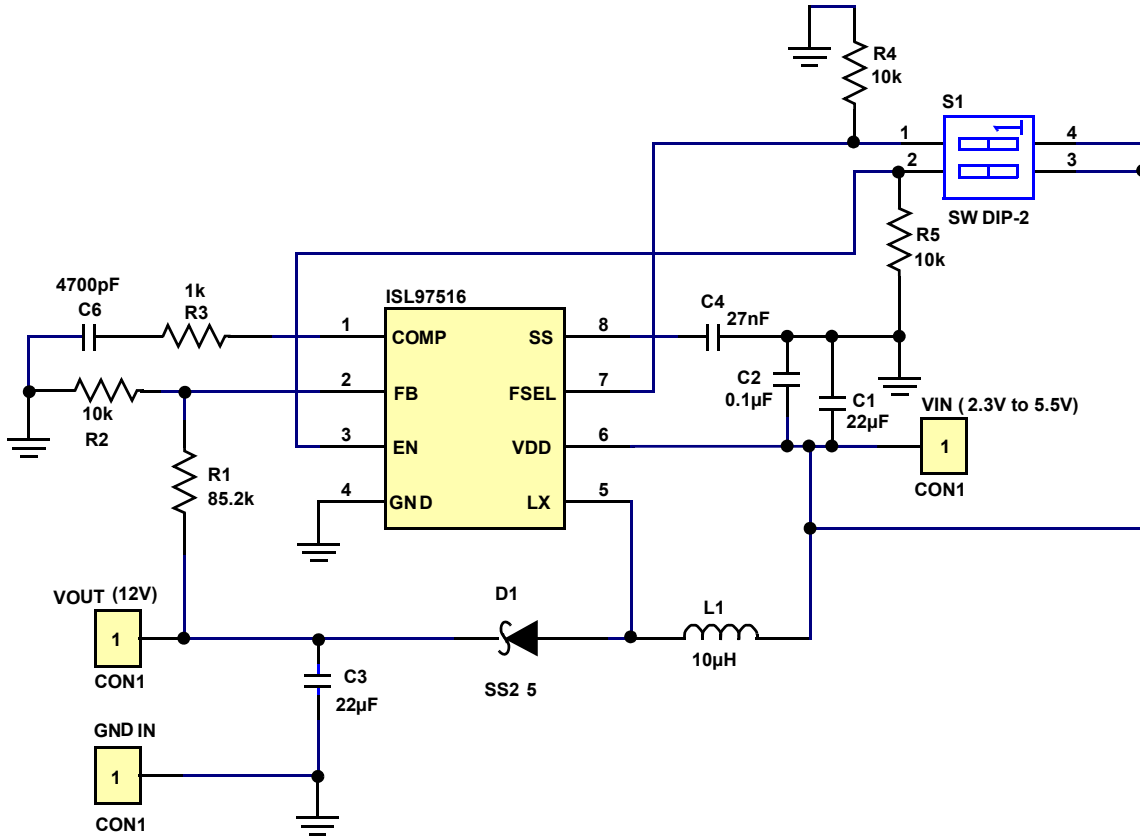
FIGURE 1. SCHEMATIC
