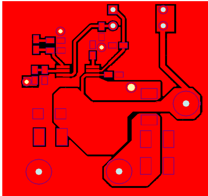
FIGURE 2. TOP LAYER
