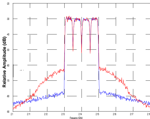
FIGURE 13. PREDISTORTION PERFORMANCE
