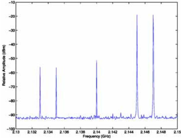
FIGURE 10A. TWO-TONE RF INPUT WITHOUT CORRECTION
