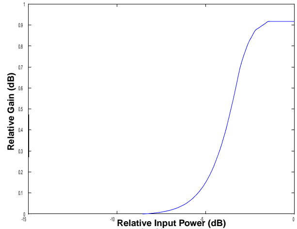
FIGURE 12A. PD AM-AM CHARACTERISTIC
