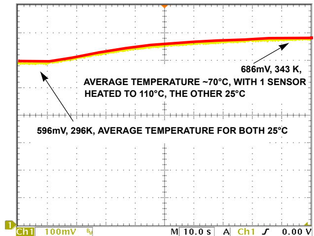
FIGURE 8. ISL71590SEH IN PARALLEL CONFIGURATION SHOWING VOLTAGE REPRESENTING THE TOTAL ARRAY CURRENT
