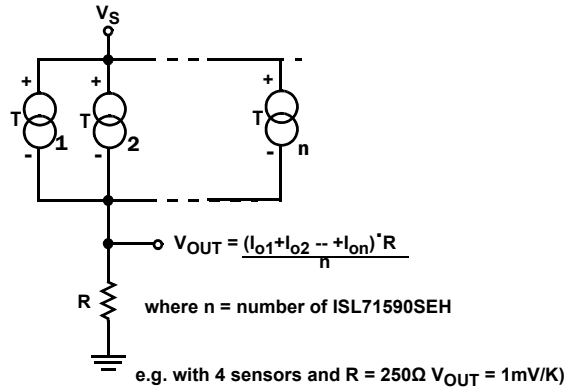
FIGURE 7. AVERAGE TEMPERATURE SENSING SCHEME
