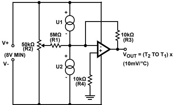
FIGURE 9. DIFFERENTIAL THERMOMETER
